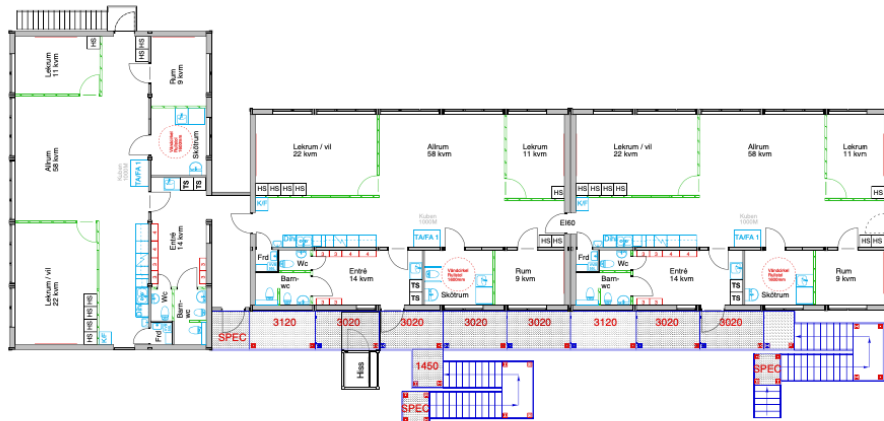
PLAN 2
