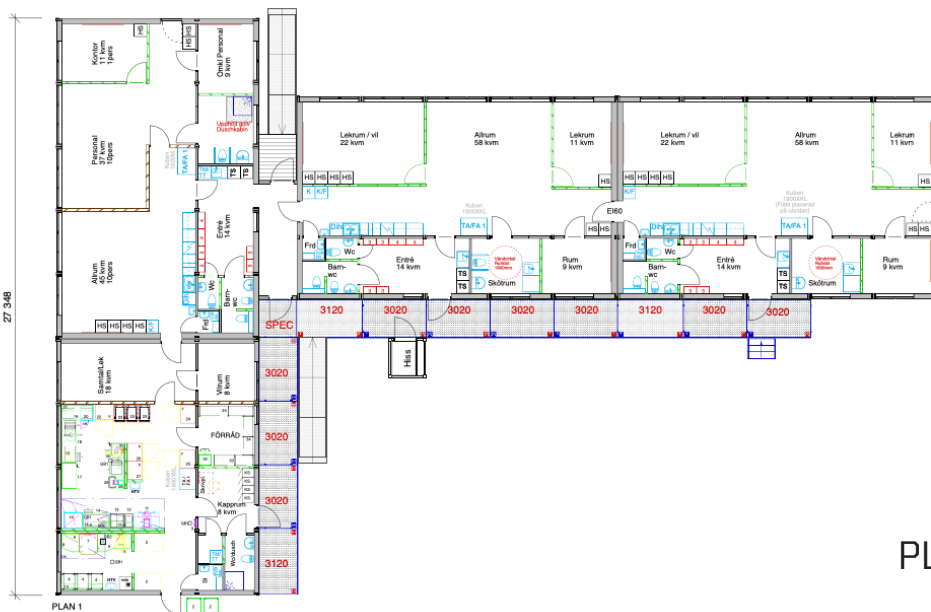
PLAN 1
